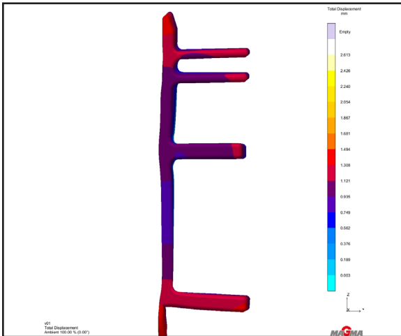
Figure 7-7: Total displacement showing casting shrinkage and distortion with a 25 times scale factor
