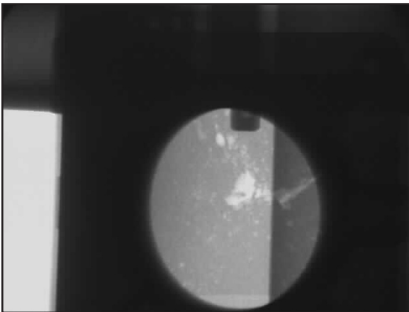
Figure 7-18C: Example radiograph of shrinkage in a thick cross-section.
