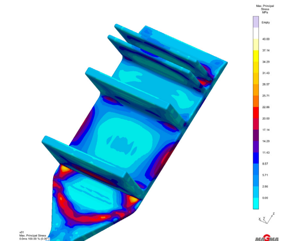
Figure 7-8: Example of the residual stresses on the casting after ejection and cooling to room temperature
