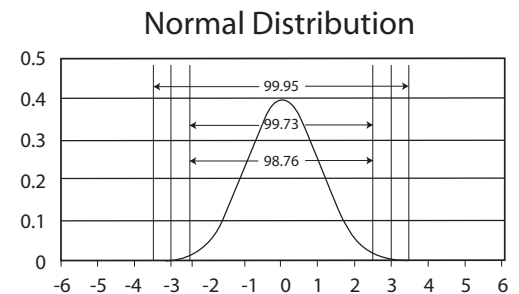
Figure 7-14: CPK indicates a normal distribution that allows within the distribution the maximum allowance of plus/minus tolerance that yields the greatest number of good parts in production. The higher the CPK number the more repeatable and accurate the process is.
